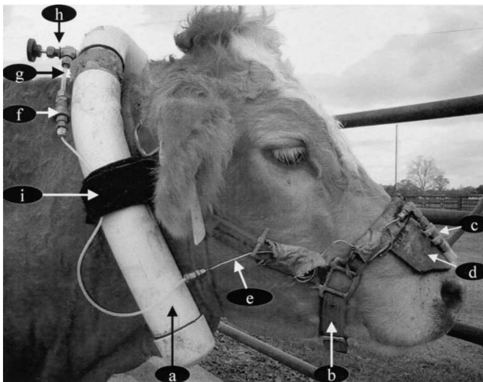
Fig. 1. Methane collection equipment as worn by a grazing cow: (a) collection canister; (b) halter; (c) filter inlet connected to capillary tubing; (d) leather muzzle protector; (e) stainless steel capillary tubing attached to halter; (f) quick-connect coupling of tubing to canister; (g) Teflon tubing between shut-off valve and quick-connect to capillary tubing; (h) shut-off valve on canister; (i) Velcro strip to anchor canister to halter.
