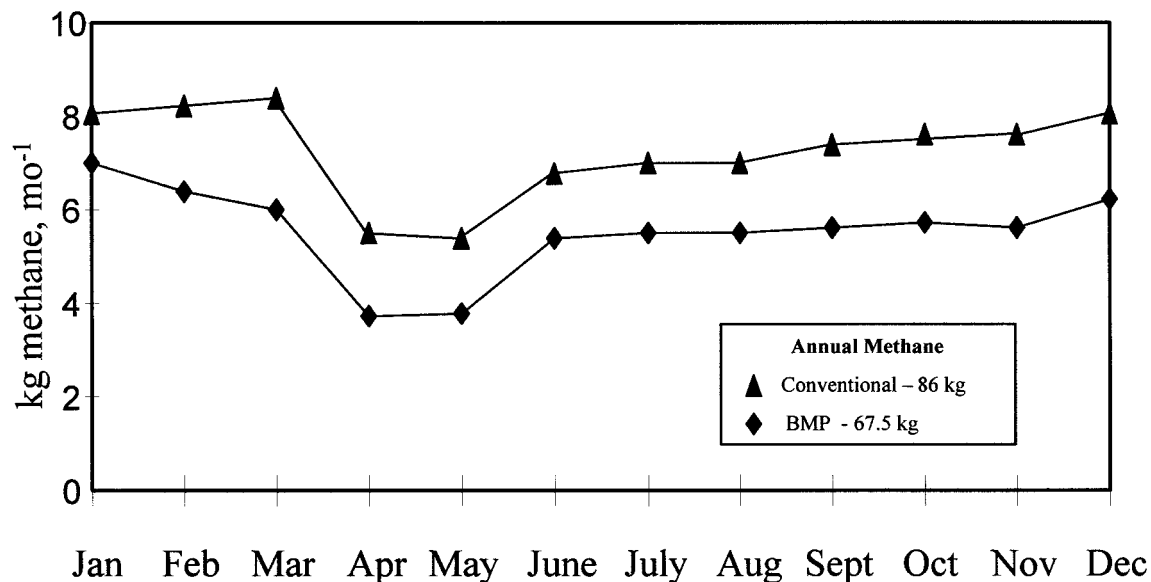
Fig. 2. Monthly methane emission projections in beef cows on best management practices (BMP) and conventional forage management systems.
